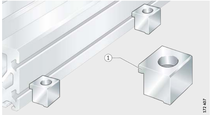
Figure 4 Fixing lug
