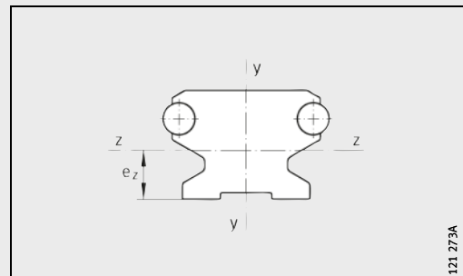
Bending axes
